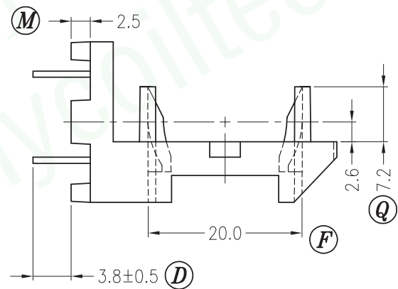
PART P-2802
