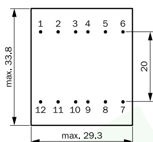
View looking onto pins
