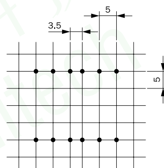
Dimensions without tolerances \pm 0.3 \text{ mm} , rights to make alterations and improvements hereby reserved
